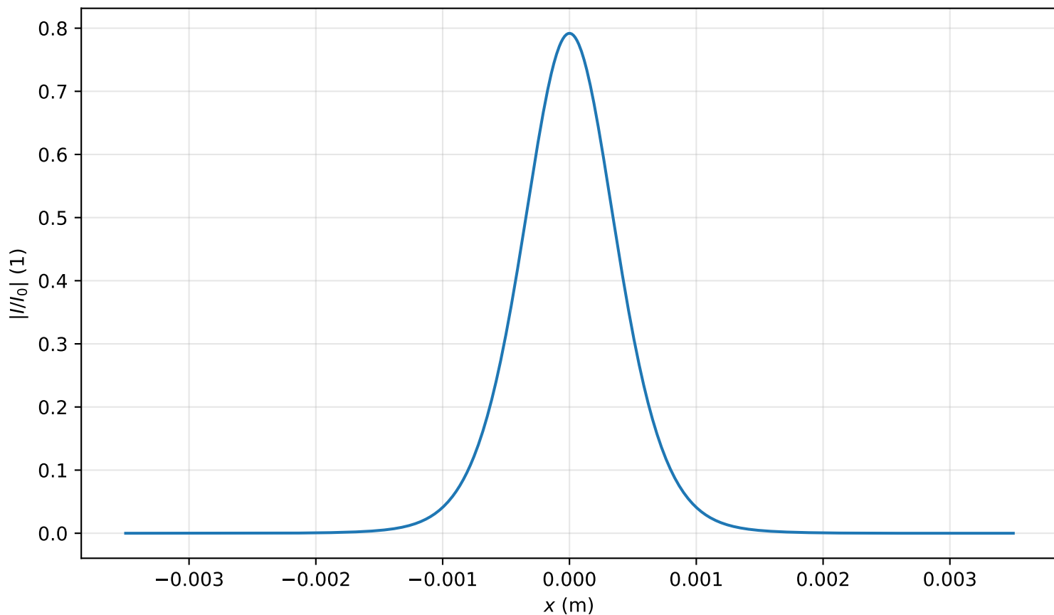
Intensity profile I(x, y = 0, z = 2.548m)/I_0 , P_{in}=0.6P_{cr} , artificial time
